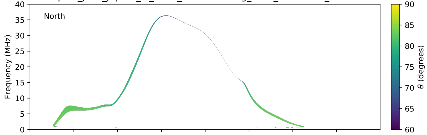
expres_juno_jupiter_io_isaac_lossc-wid1deg_3kev_20181130_v01.cdf
