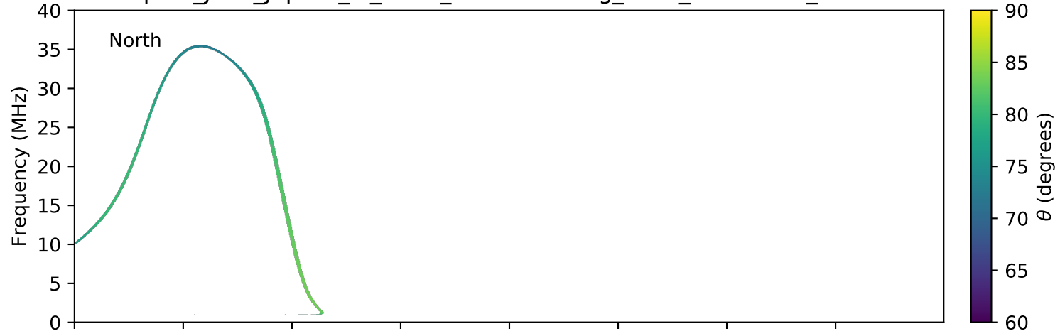
expres_juno_jupiter_io_isaac_lossc-wid1deg_3kev_20181127_v01.cdf
