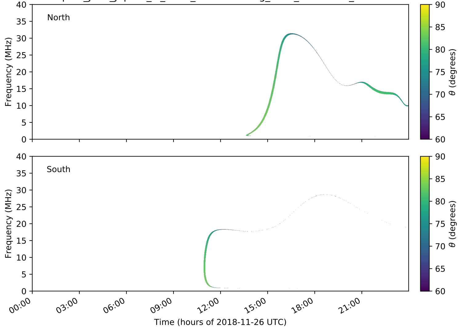
expres_juno_jupiter_io_isaac_lossc-wid1deg_3kev_20181126_v01.cdf
