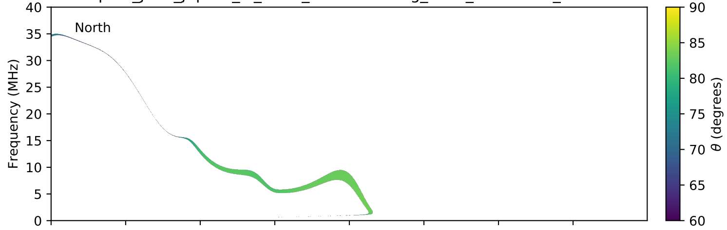
expres_juno_jupiter_io_isaac_lossc-wid1deg_3kev_20181125_v01.cdf
