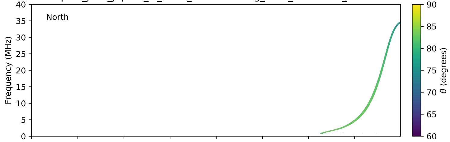
expres_juno_jupiter_io_isaac_lossc-wid1deg_3kev_20181124_v01.cdf
