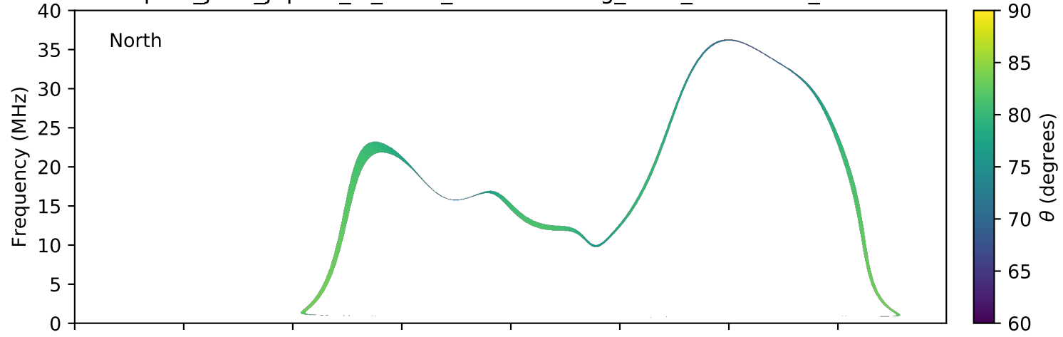
expres_juno_jupiter_io_isaac_lossc-wid1deg_3kev_20181121_v01.cdf
