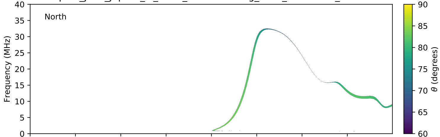
expres_juno_jupiter_io_isaac_lossc-wid1deg_3kev_20181119_v01.cdf
