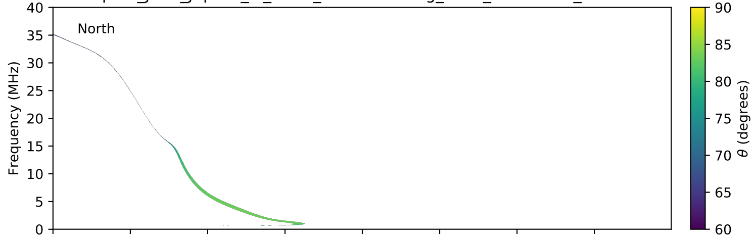
expres_juno_jupiter_io_isaac_lossc-wid1deg_3kev_20181118_v01.cdf
