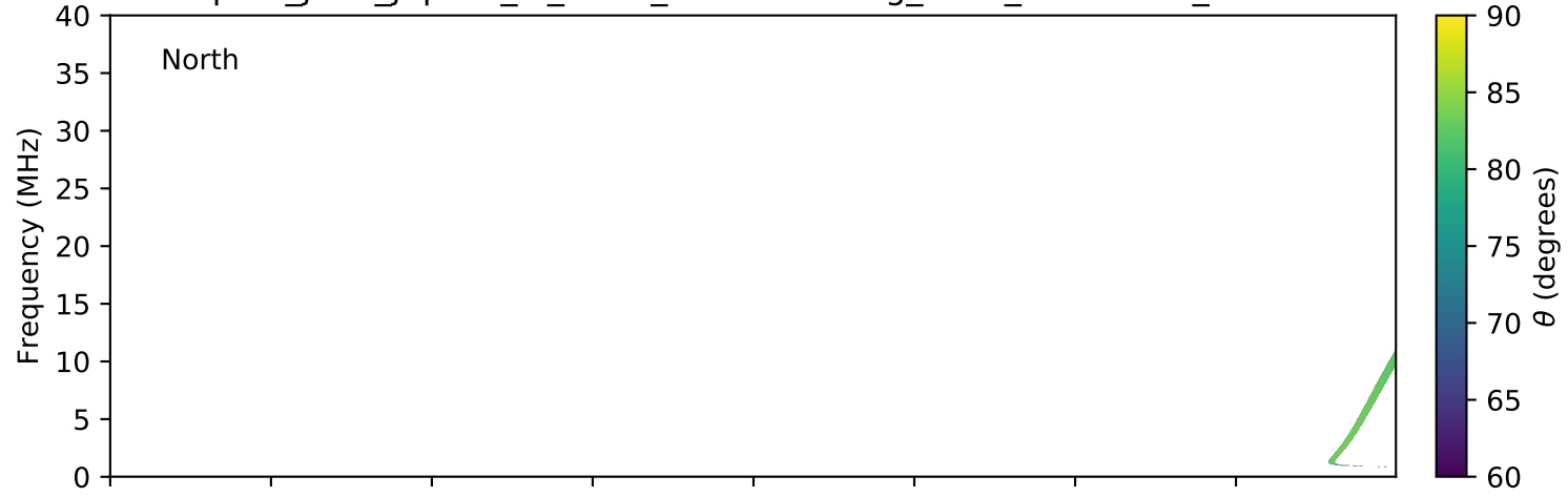
expres_juno_jupiter_io_isaac_lossc-wid1deg_3kev_20181115_v01.cdf
