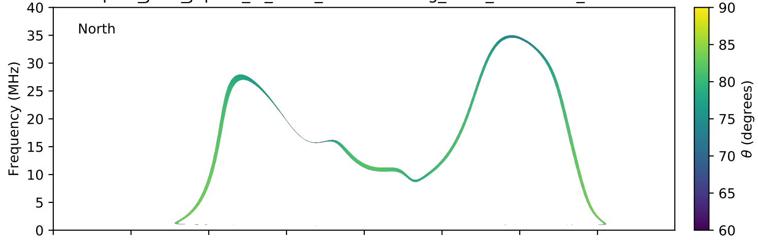
expres_juno_jupiter_io_isaac_lossc-wid1deg_3kev_20181114_v01.cdf
