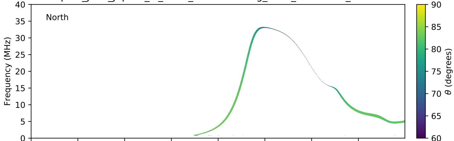
expres_juno_jupiter_io_isaac_lossc-wid1deg_3kev_20181112_v01.cdf
