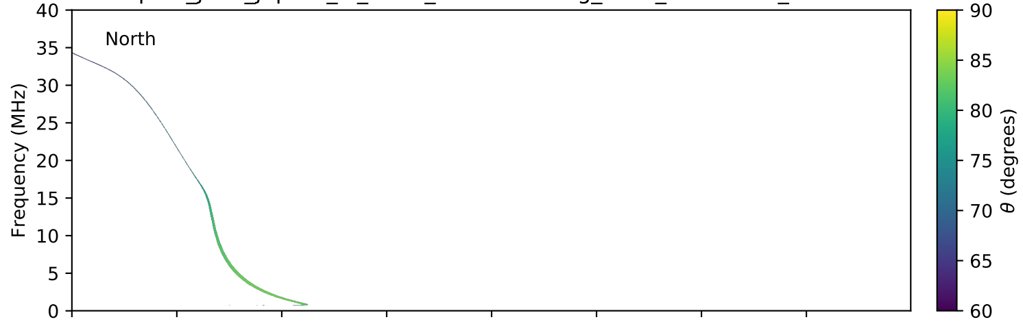
expres_juno_jupiter_io_isaac_lossc-wid1deg_3kev_20181111_v01.cdf
