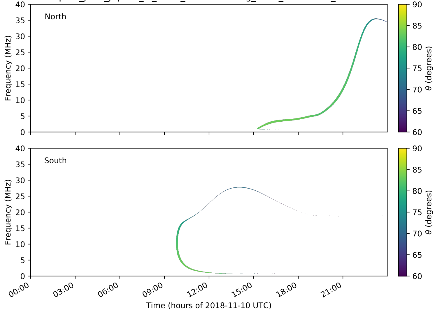
expres_juno_jupiter_io_isaac_lossc-wid1deg_3kev_20181110_v01.cdf
