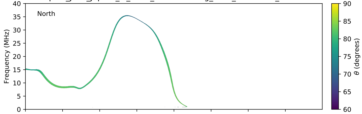
expres_juno_jupiter_io_isaac_lossc-wid1deg_3kev_20181109_v01.cdf
