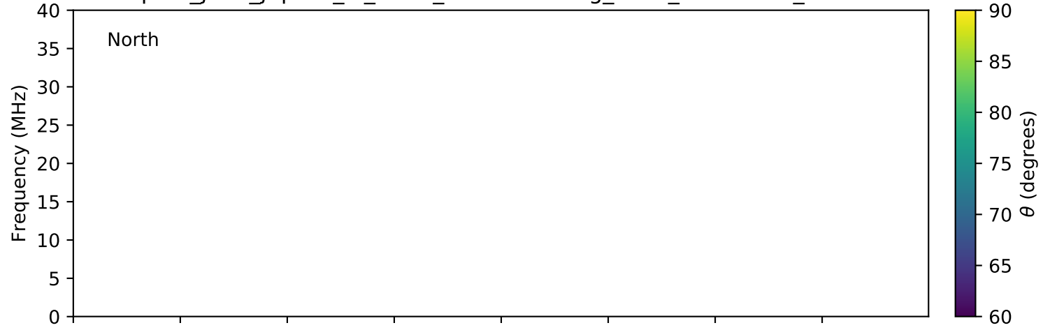
expres_juno_jupiter_io_isaac_lossc-wid1deg_3kev_20181106_v01.cdf
