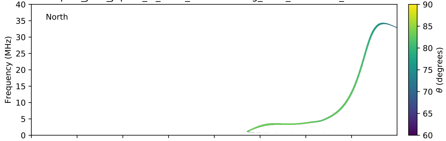
expres_juno_jupiter_io_isaac_lossc-wid1deg_3kev_20181103_v01.cdf
