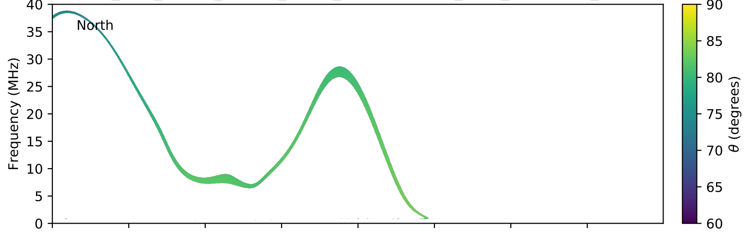
expres_juno_jupiter_europa_jrm09_lossc-wid1deg_3kev_20181130_v01.cdf
