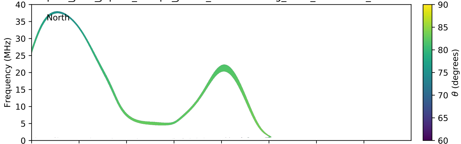
expres_juno_jupiter_europa_jrm09_lossc-wid1deg_3kev_20181125_v01.cdf
