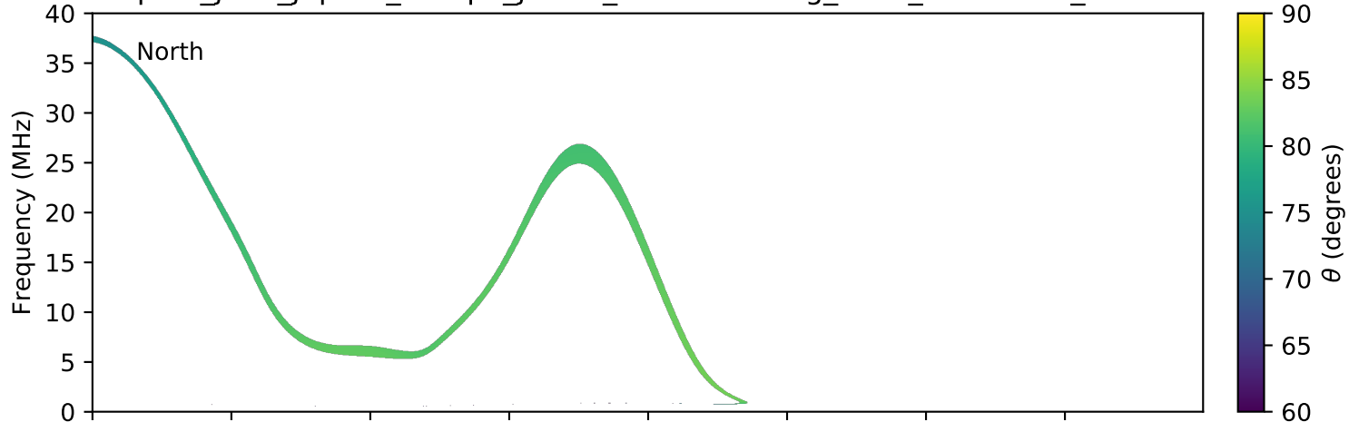
expres_juno_jupiter_europa_jrm09_lossc-wid1deg_3kev_20181123_v01.cdf
