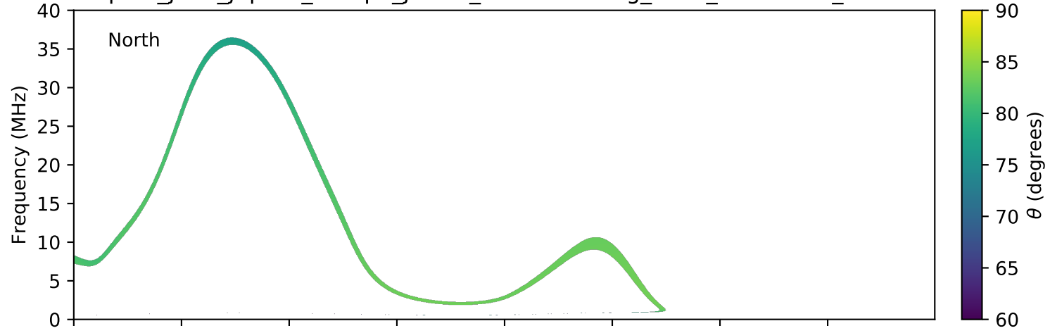
expres_juno_jupiter_europa_jrm09_lossc-wid1deg_3kev_20181122_v01.cdf
