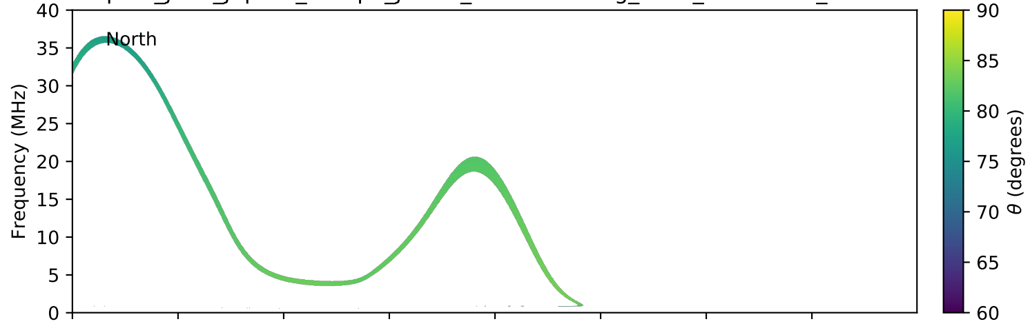
expres_juno_jupiter_europa_jrm09_lossc-wid1deg_3kev_20181118_v01.cdf
