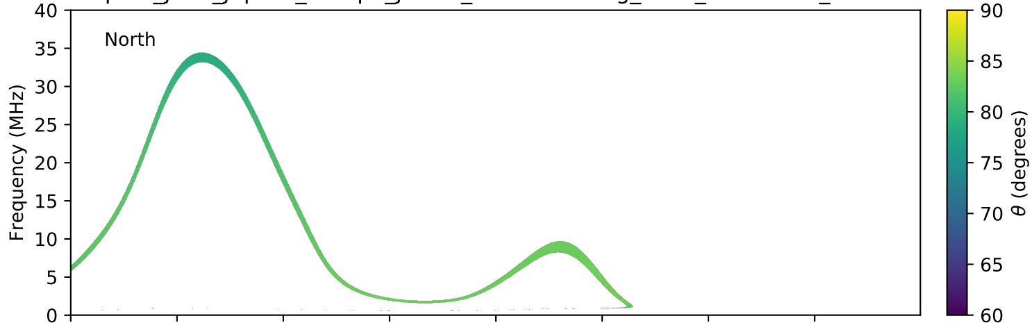
expres_juno_jupiter_europa_jrm09_lossc-wid1deg_3kev_20181115_v01.cdf
