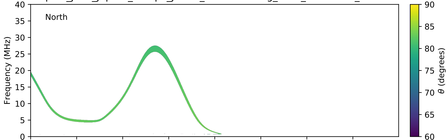
expres_juno_jupiter_europa_jrm09_lossc-wid1deg_3kev_20181114_v01.cdf
