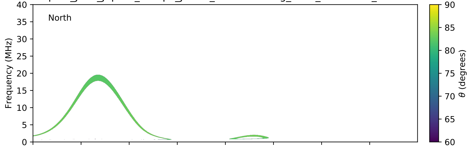
expres_juno_jupiter_europa_jrm09_lossc-wid1deg_3kev_20181103_v01.cdf
