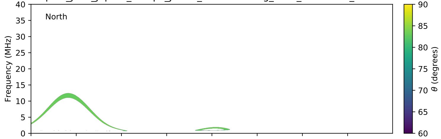
expres_juno_jupiter_europa_jrm09_lossc-wid1deg_3kev_20181101_v01.cdf
