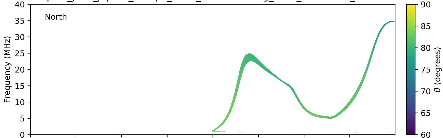
expres_juno_jupiter_europa_isaac_lossc-wid1deg_3kev_20181129_v01.cdf
