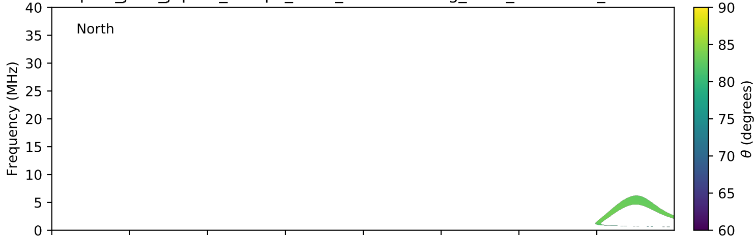
expres_juno_jupiter_europa_isaac_lossc-wid1deg_3kev_20181125_v01.cdf
