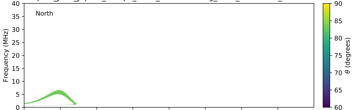
expres_juno_jupiter_europa_isaac_lossc-wid1deg_3kev_20181120_v01.cdf
