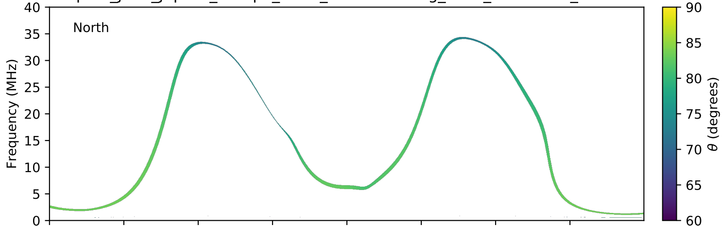
expres_juno_jupiter_europa_isaac_lossc-wid1deg_3kev_20181119_v01.cdf
