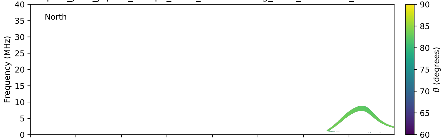
expres_juno_jupiter_europa_isaac_lossc-wid1deg_3kev_20181118_v01.cdf
