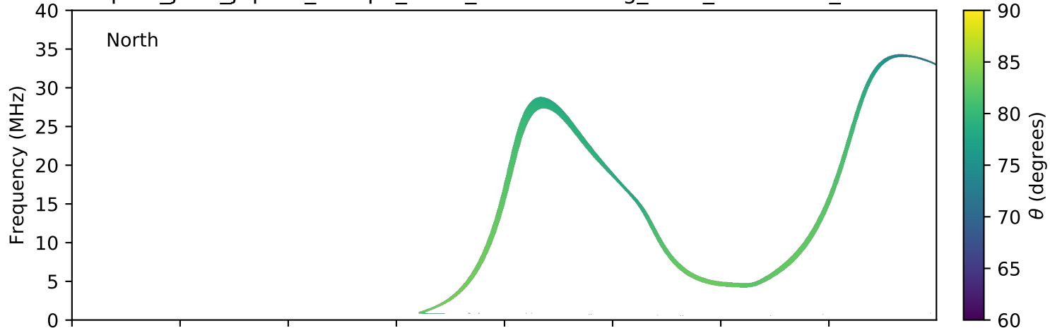
expres_juno_jupiter_europa_isaac_lossc-wid1deg_3kev_20181115_v01.cdf
