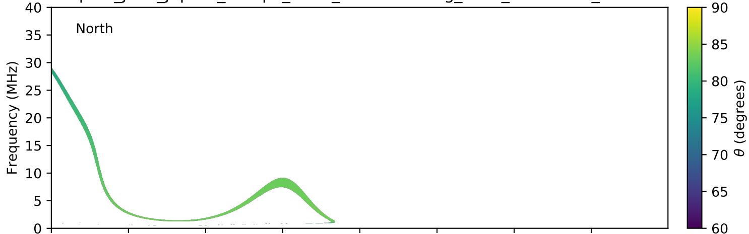
expres_juno_jupiter_europa_isaac_lossc-wid1deg_3kev_20181109_v01.cdf
