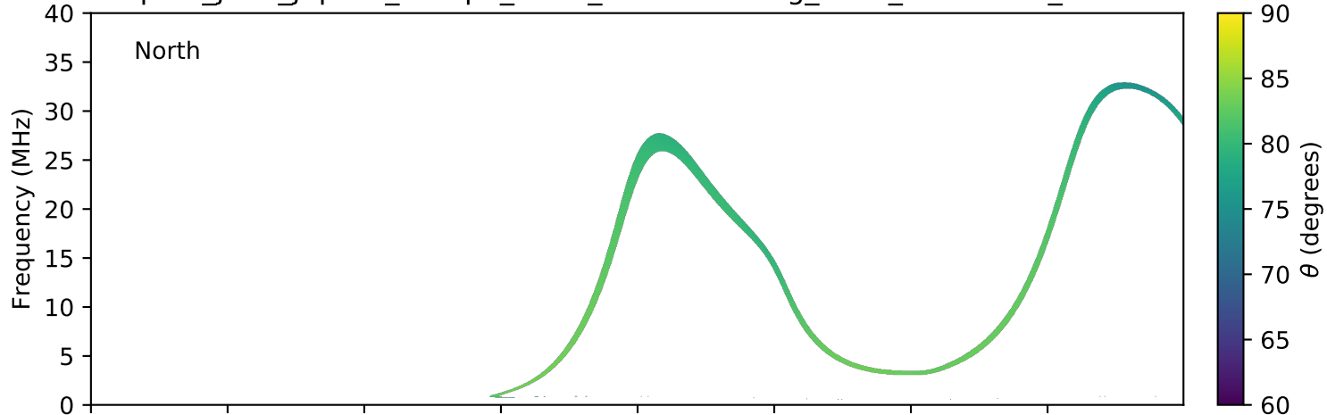
expres_juno_jupiter_europa_isaac_lossc-wid1deg_3kev_20181108_v01.cdf
