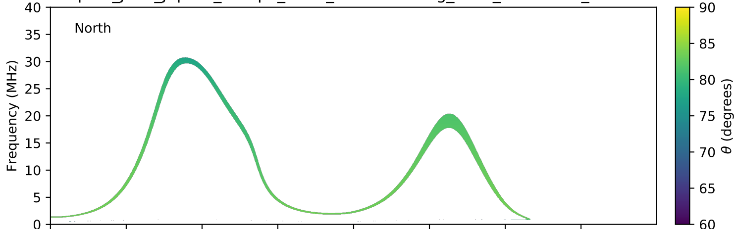
expres_juno_jupiter_europa_isaac_lossc-wid1deg_3kev_20181105_v01.cdf
