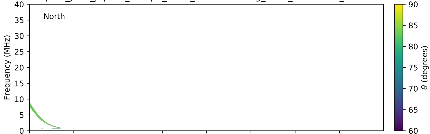
expres_juno_jupiter_europa_isaac_lossc-wid1deg_3kev_20181102_v01.cdf
