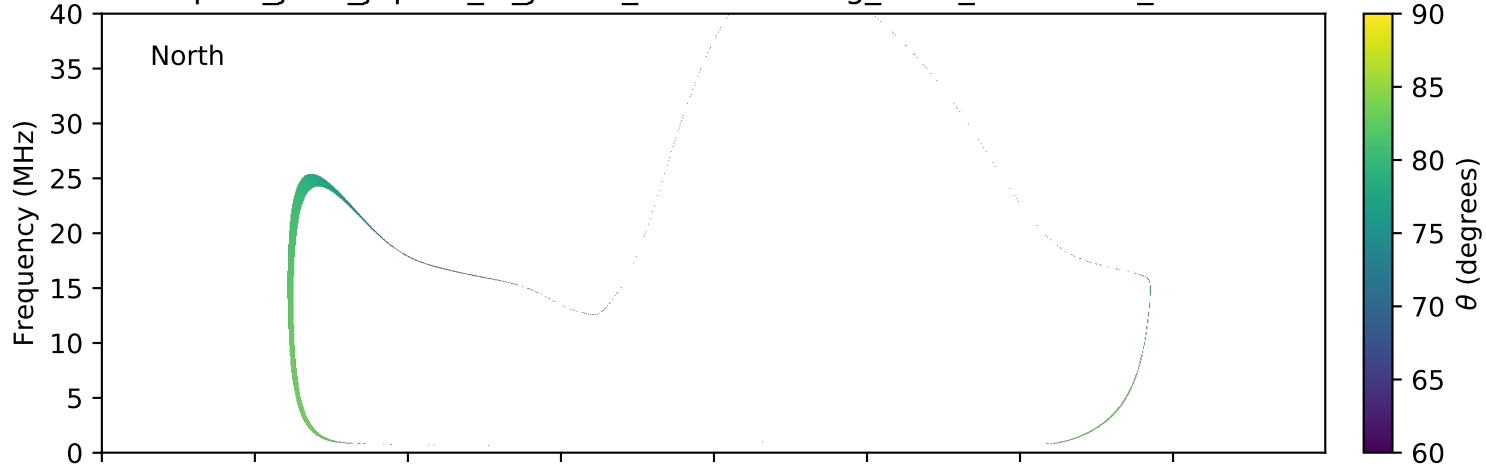
expres_juno_jupiter_io_jrm09_lossc-wid1deg_3kev_20181029_v01.cdf
