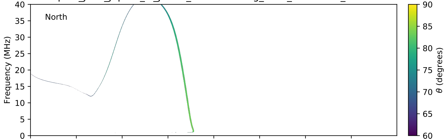
expres_juno_jupiter_io_jrm09_lossc-wid1deg_3kev_20181026_v01.cdf
