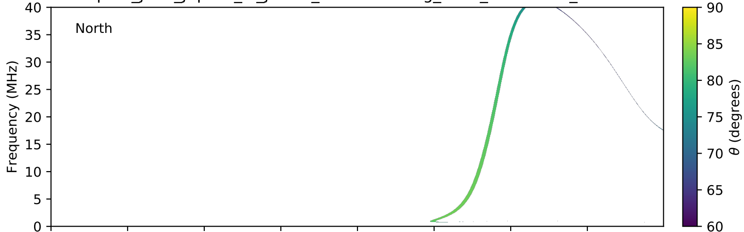
expres_juno_jupiter_io_jrm09_lossc-wid1deg_3kev_20181018_v01.cdf
