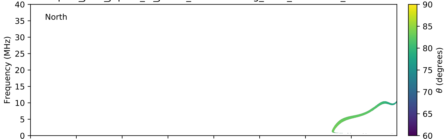
expres_juno_jupiter_io_jrm09_lossc-wid1deg_3kev_20181016_v01.cdf
