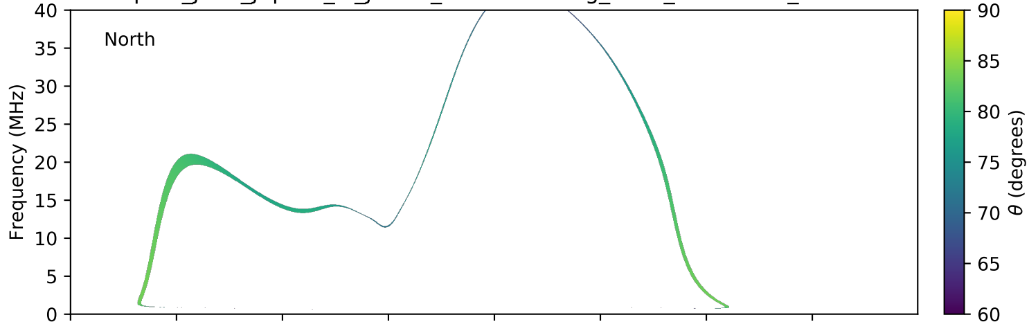
expres_juno_jupiter_io_jrm09_lossc-wid1deg_3kev_20181015_v01.cdf
