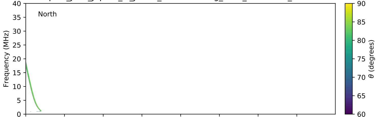
expres_juno_jupiter_io_jrm09_lossc-wid1deg_3kev_20181014_v01.cdf
