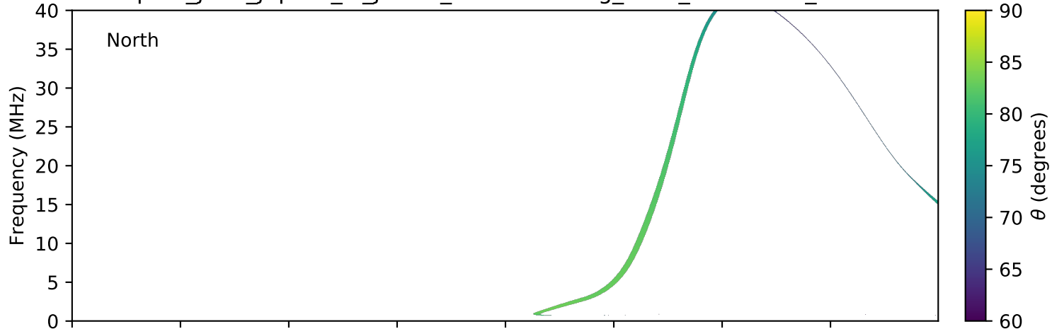
expres_juno_jupiter_io_jrm09_lossc-wid1deg_3kev_20181011_v01.cdf
