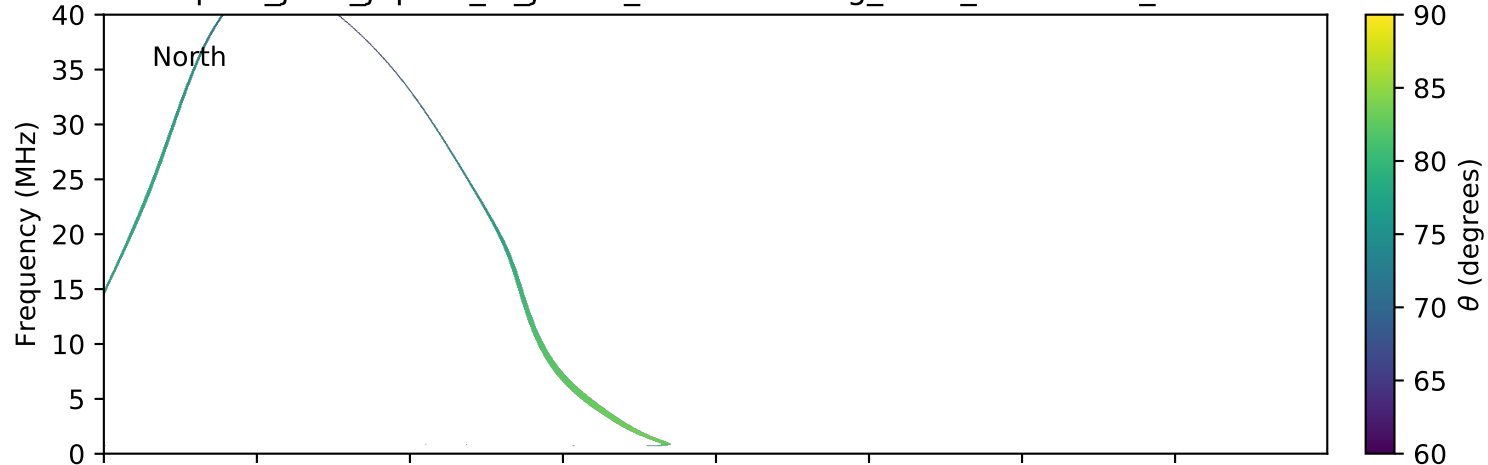
expres_juno_jupiter_io_jrm09_lossc-wid1deg_3kev_20181010_v01.cdf
