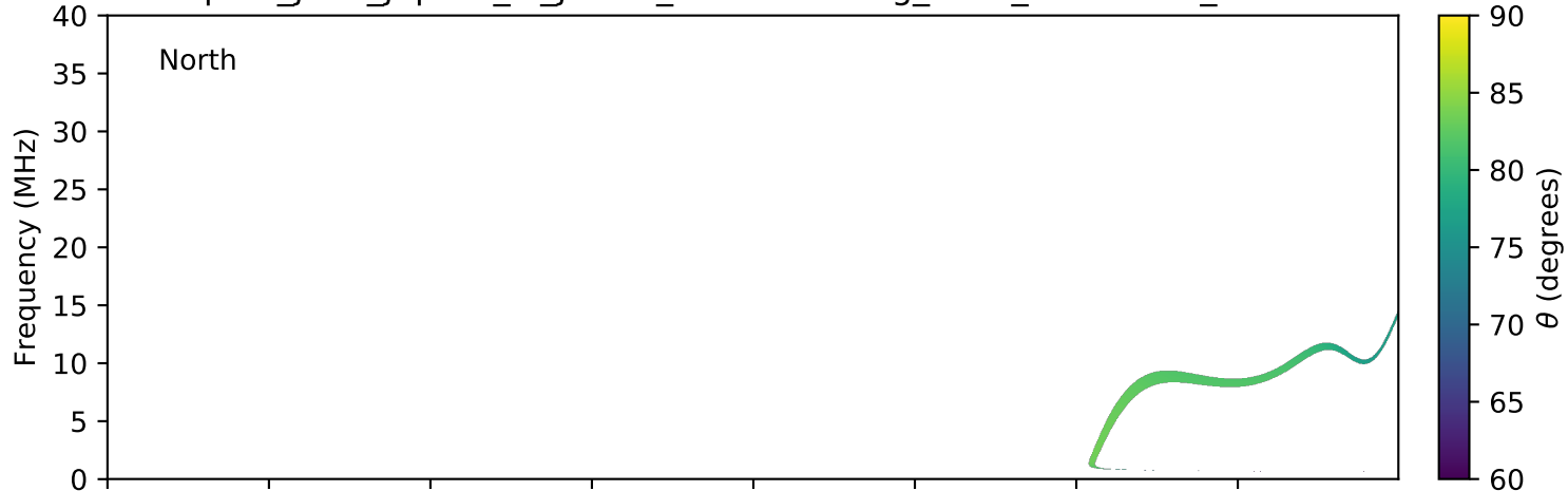
expres_juno_jupiter_io_jrm09_lossc-wid1deg_3kev_20181009_v01.cdf
