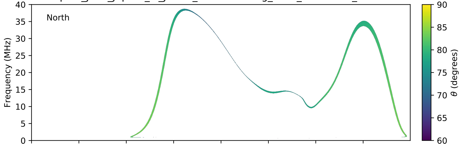
expres_juno_jupiter_io_jrm09_lossc-wid1deg_3kev_20181006_v01.cdf
