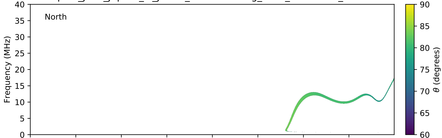
expres_juno_jupiter_io_jrm09_lossc-wid1deg_3kev_20181002_v01.cdf
