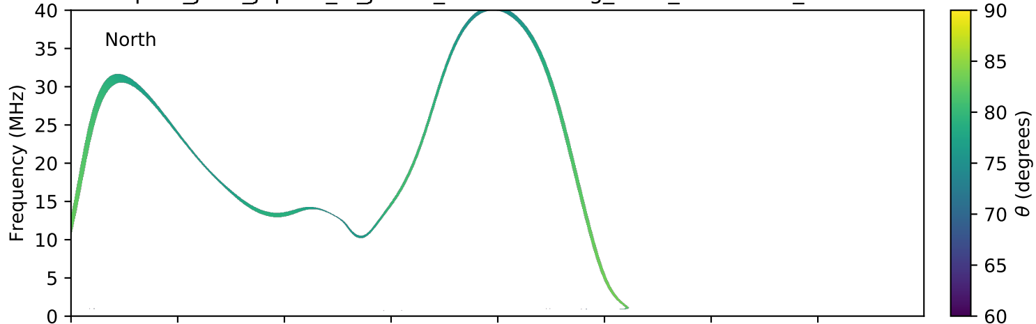
expres_juno_jupiter_io_jrm09_lossc-wid1deg_3kev_20181001_v01.cdf
