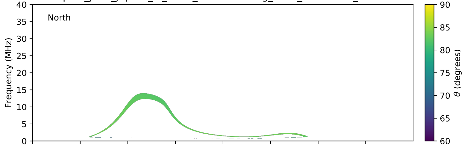
expres_juno_jupiter_io_isaac_lossc-wid1deg_3kev_20181031_v01.cdf
