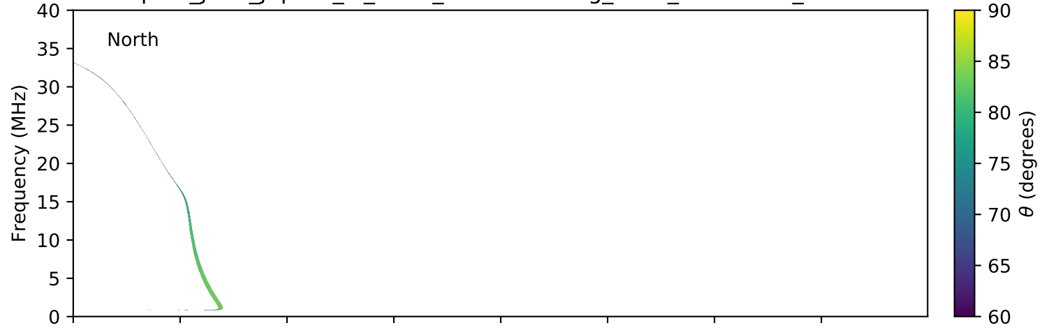
expres_juno_jupiter_io_isaac_lossc-wid1deg_3kev_20181028_v01.cdf
