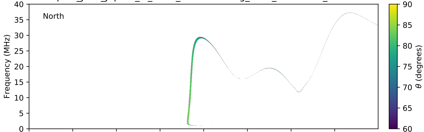
expres_juno_jupiter_io_isaac_lossc-wid1deg_3kev_20181027_v01.cdf
